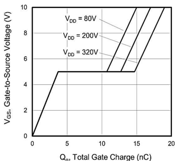
Figure 8. Gate Charge
