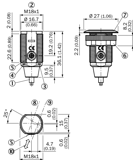
GRTB18S, plastic, cable, straight, adjustable
