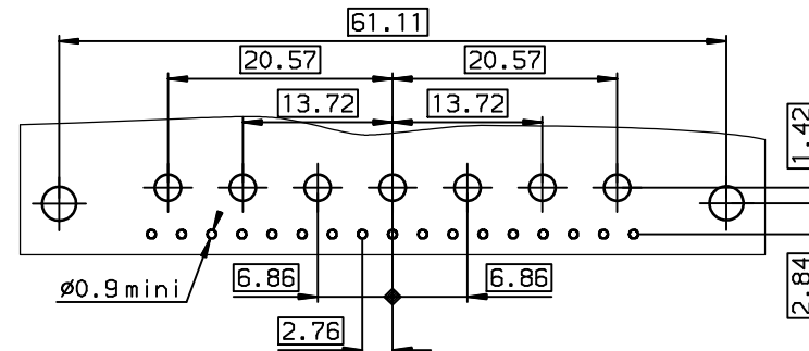
LAYOUT DIMENSIONS (after plating) CONNECTOR SIDE VIEW
