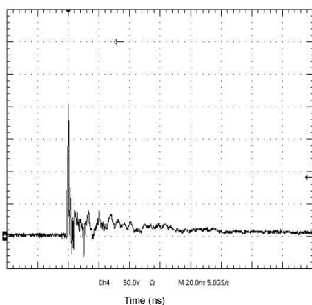
Fig.3 IEC61000-4-2 +8kV Contact Discharge
