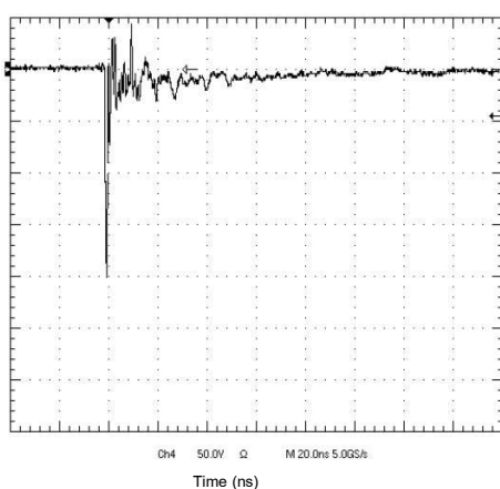
Fig.4 IEC61000-4-2 -8kV Contact Discharge
