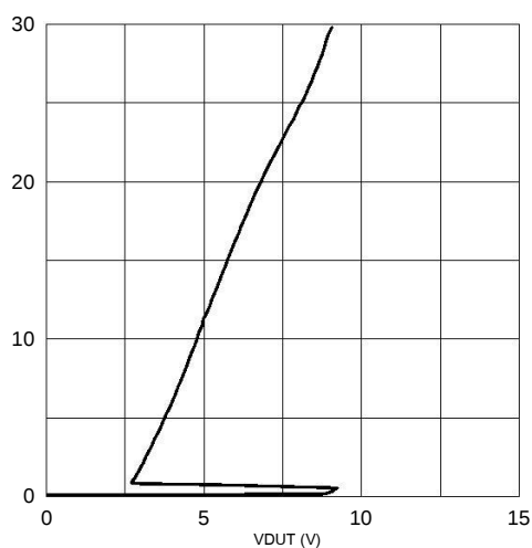
Fig.5 Transmission Line Pulse (tp=100ns)
