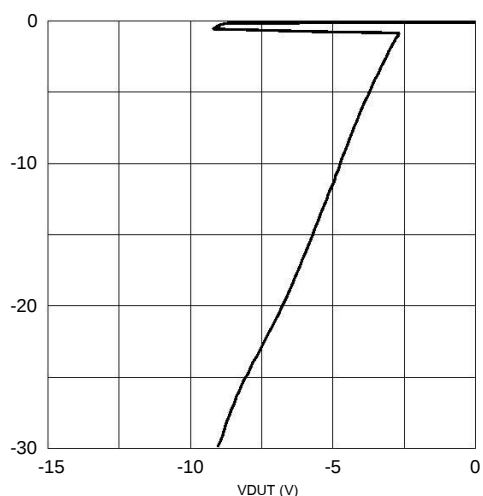
Fig.6 Transmission Line Pulse (tp=100ns)
