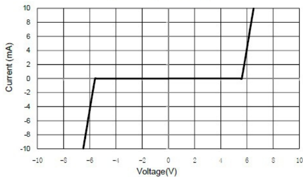
Fig 5 Voltage Sweeping
