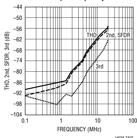
2nd, 3rd and SFDR vs Input Frequency
