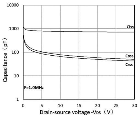
Figure 7. Capacitance Characteristics
