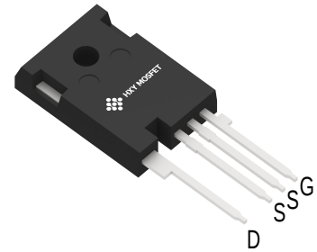
TO-247H-4L (TO-247H-4)
