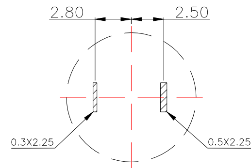
PCB.WELDING DRAWING
