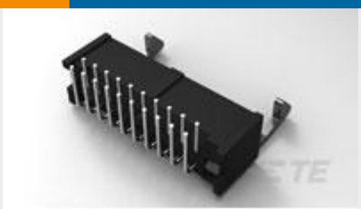
TE Part #2-1761607-9 IDC LOW PRO HDR 26P RA LG LAT
