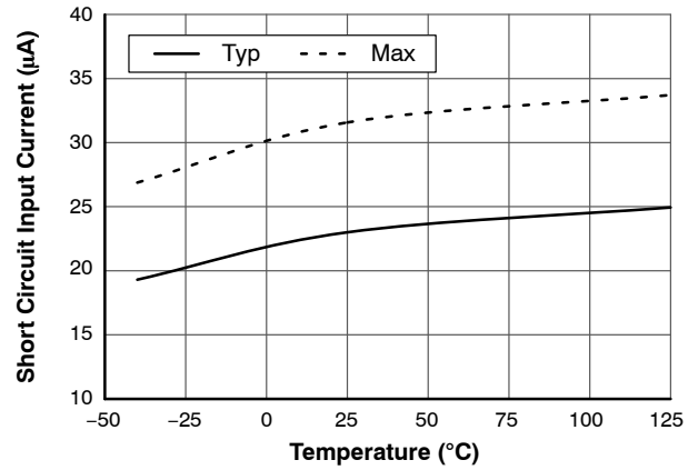
Figure 13. I_{CSCIN} vs. Temperature
