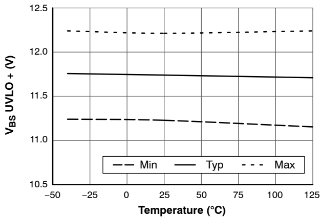
Figure 6. V_{BS} UVLO (+) vs. Temperature
