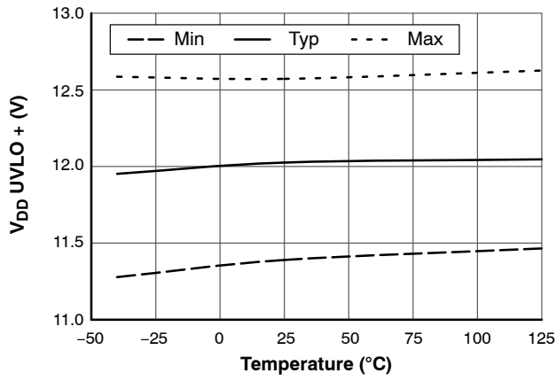
Figure 4. V_{DD} UVLO (+) vs. Temperature
