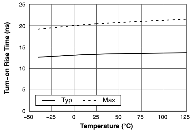
Figure 15. Turn-on Rising Time vs. Temperature
