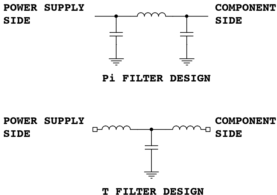
Figure 5–2. Filter Designs
