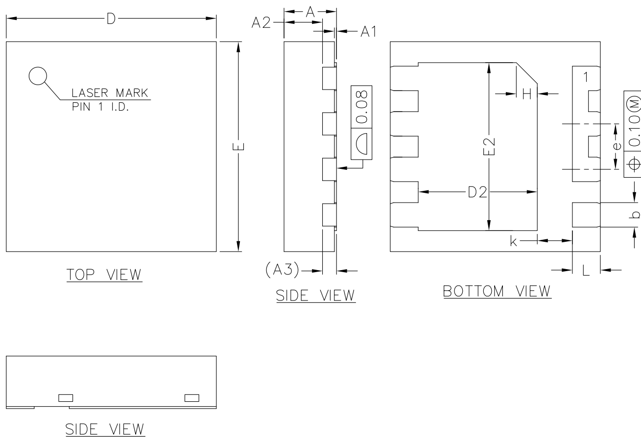
DFN3x3
