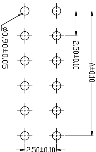
PCB LAYOUT
