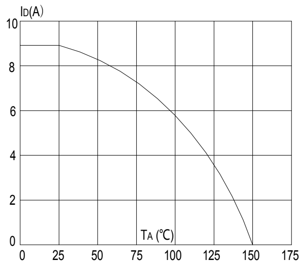
Figure 10: Maximum Continuous Drain Current vs. Ambient Temperature
