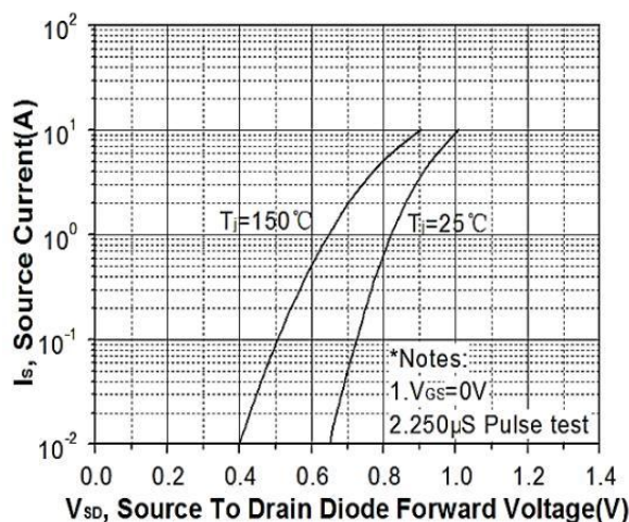
Figure 5. Forward characteristics of reverse diode
