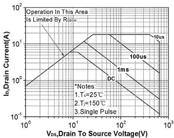
Figure 9. Safe operating area(TO-252)
