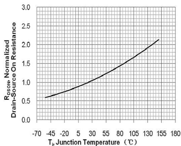
Figure 3. R_DS(ON) vs Junction Temperature
