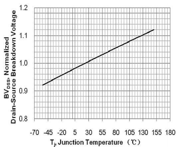
Figure 1. BVDSS vs Junction Temperature
