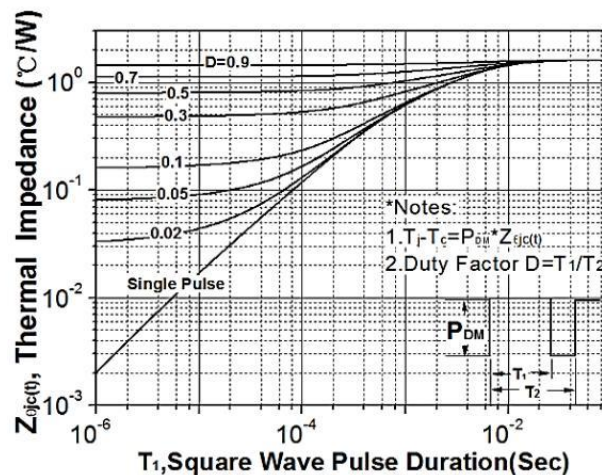
Figure 10. Transient thermal impedance (TO-252)
