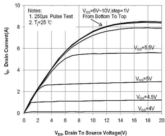
Figure 8. Output characteristics
