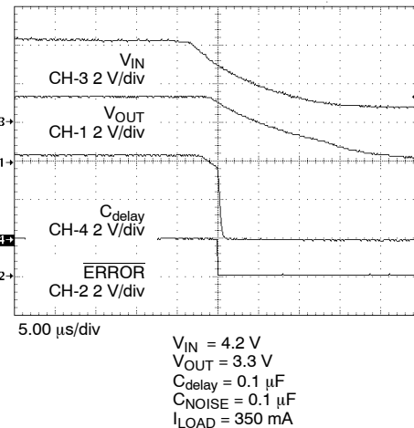
Turn-Off Sequence
