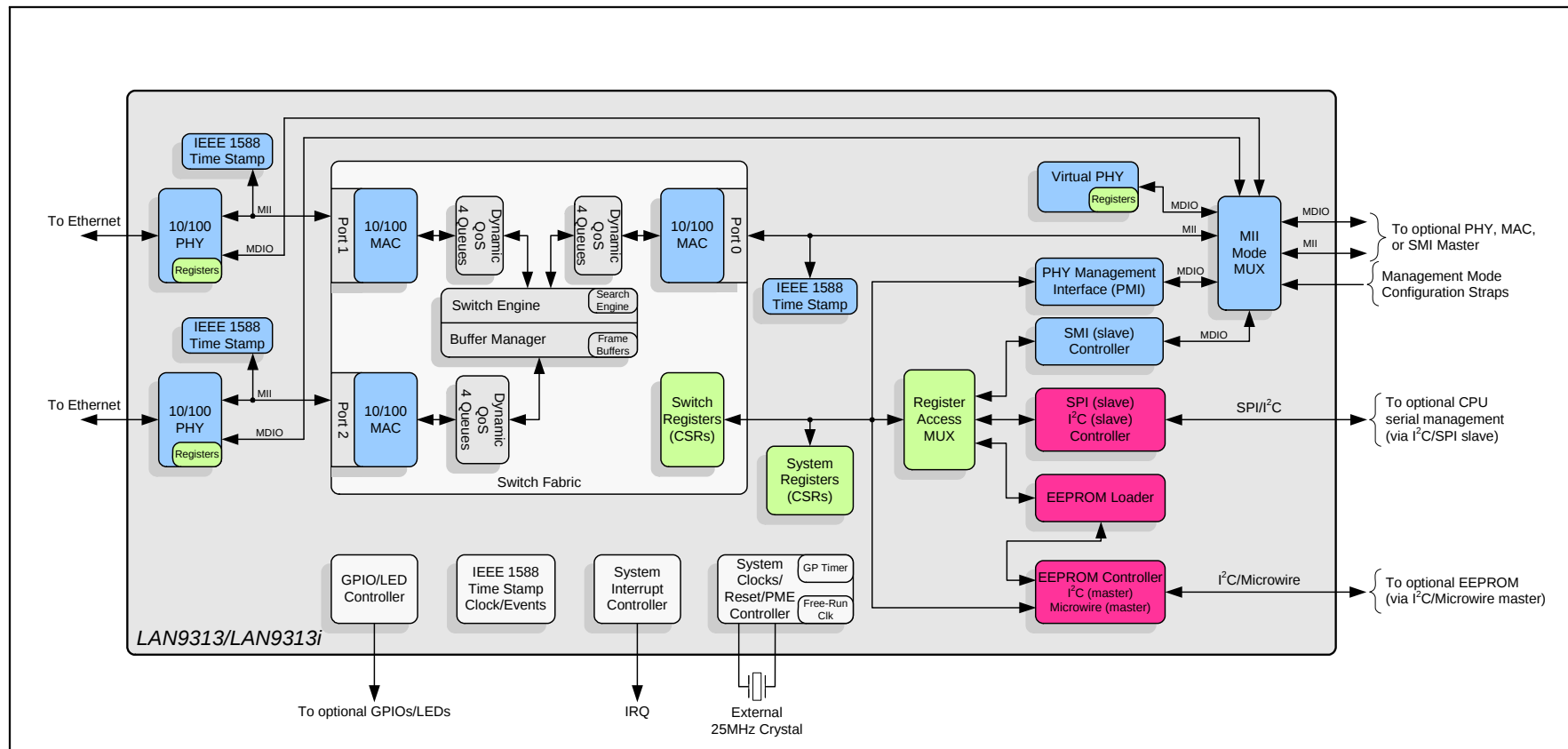
FIGURE 2-1: INTERNAL LAN9313/LAN9313i BLOCK DIAGRAM
