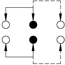
SCHEMATIC (NON-SHORTING)
