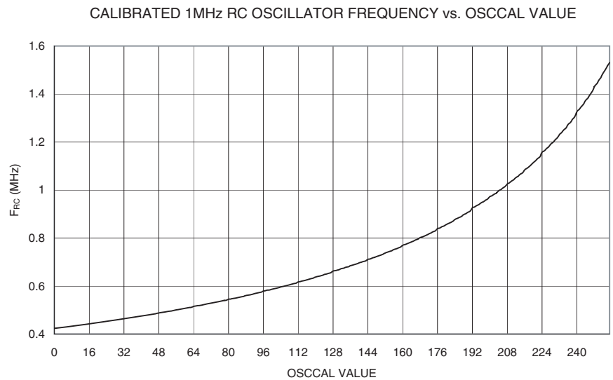
Figure 205. Calibrated 1 MHz RC Oscillator Frequency vs. OSCCAL Value
