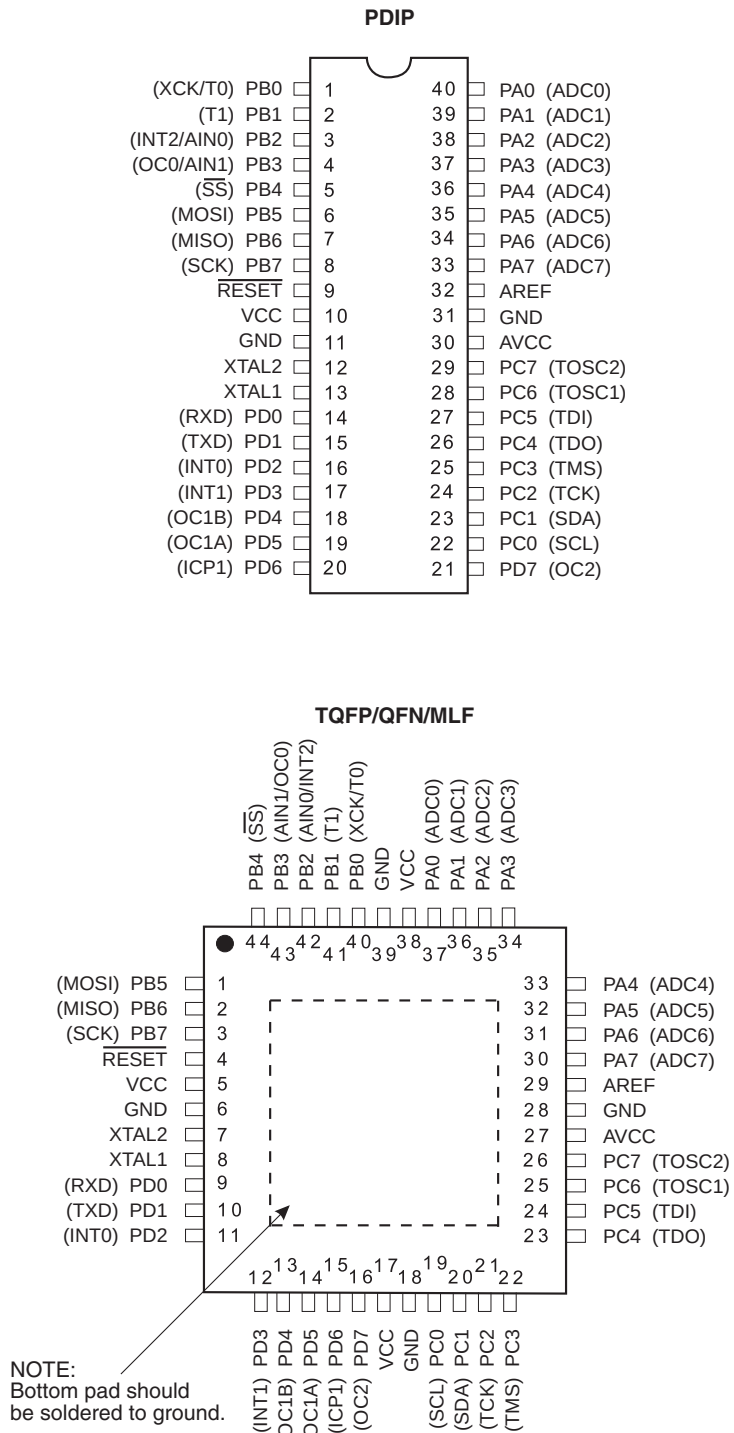
Figure 1. Pinout ATmega16
