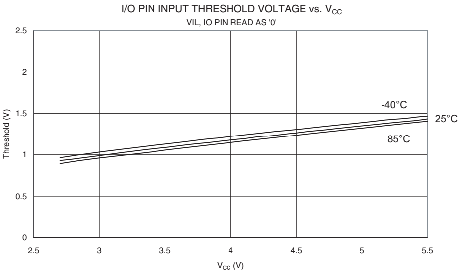
Figure 183. I/O Pin Input Threshold Voltage vs. V_{CC} ( V_{IL} , I/O Pin Read As '0')
