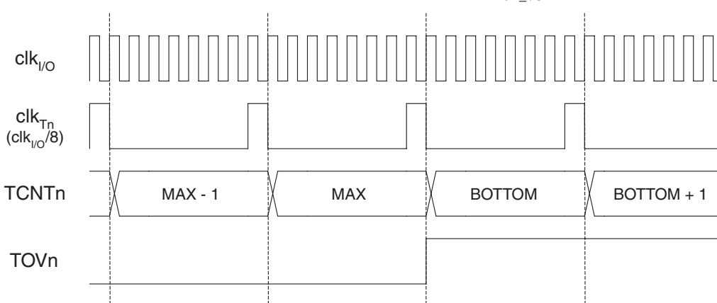
Figure 61. Timer/Counter Timing Diagram, with Prescaler ( f_{\text{clk}_{I/O}}/8 )
