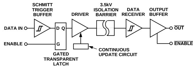
Figure 1. Simplified Block Diagram
