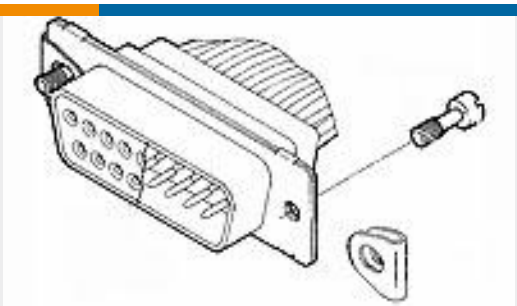
TE Part #211883-5 SCREW RETAINER KIT,AMPLITE
