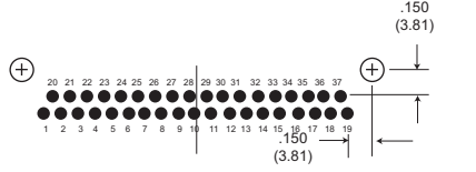
37 Contacts
