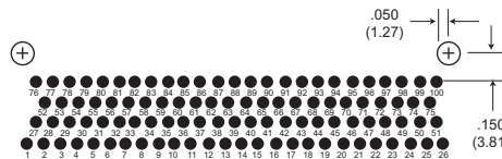
100 Contacts
