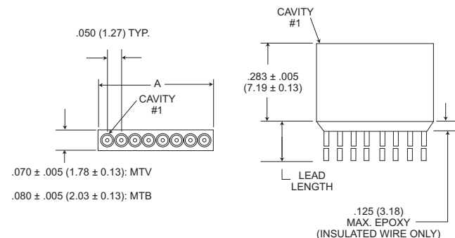
Plug
