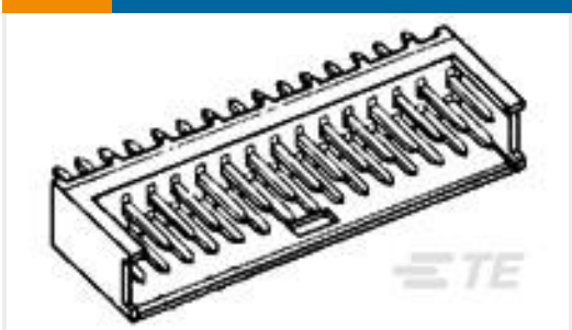
TE Part #280509-2 2X09 POS .100DR MODU-
