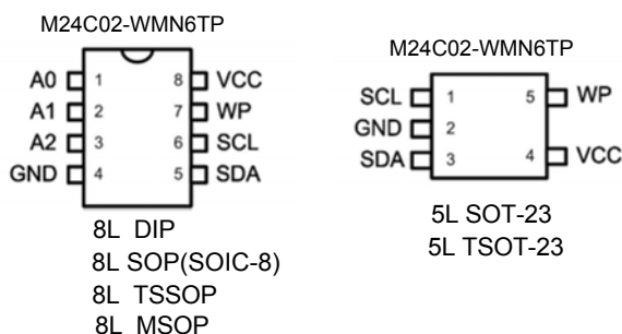
Figure 1: Package types
