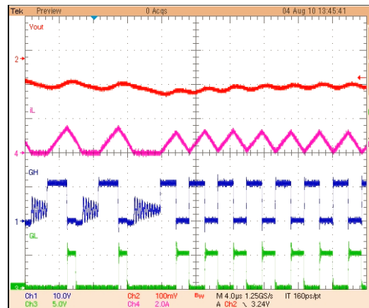
Figure 1: PFM to PWM Transition
