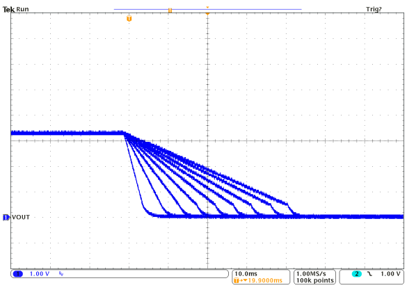
Figure 12: Ramp-Down Rate Dynamic Sweep
