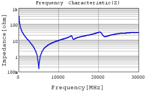
GJM0335G2A5R3WB01 |Z| DCOV, 25degC
