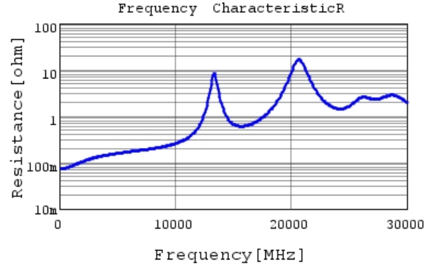
GJM0335G2A5R3WB01 R DCOV, 25degC
