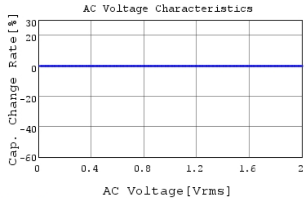
GJM0335G2A5R3WB01 C-AC Voltage capchange, Dc
