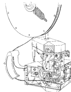
AMP-O-LECTRIC Model "G" Terminating Machines 354500-[ ] (409-5842) or 356462-[ ] (408-4357)
