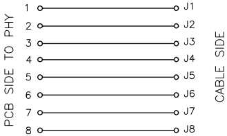
BACK VIEW
