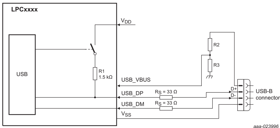
Fig 49. USB interface on a self-powered device where USB_VBUS = 5 V
