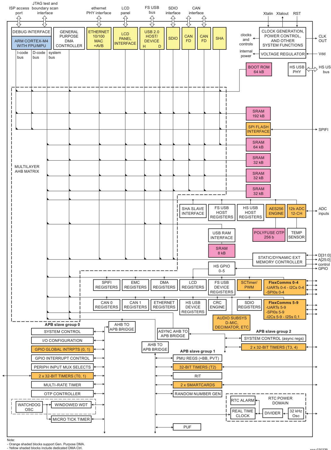
Fig 4. LPC540xx/LPC54S0xx Block diagram
