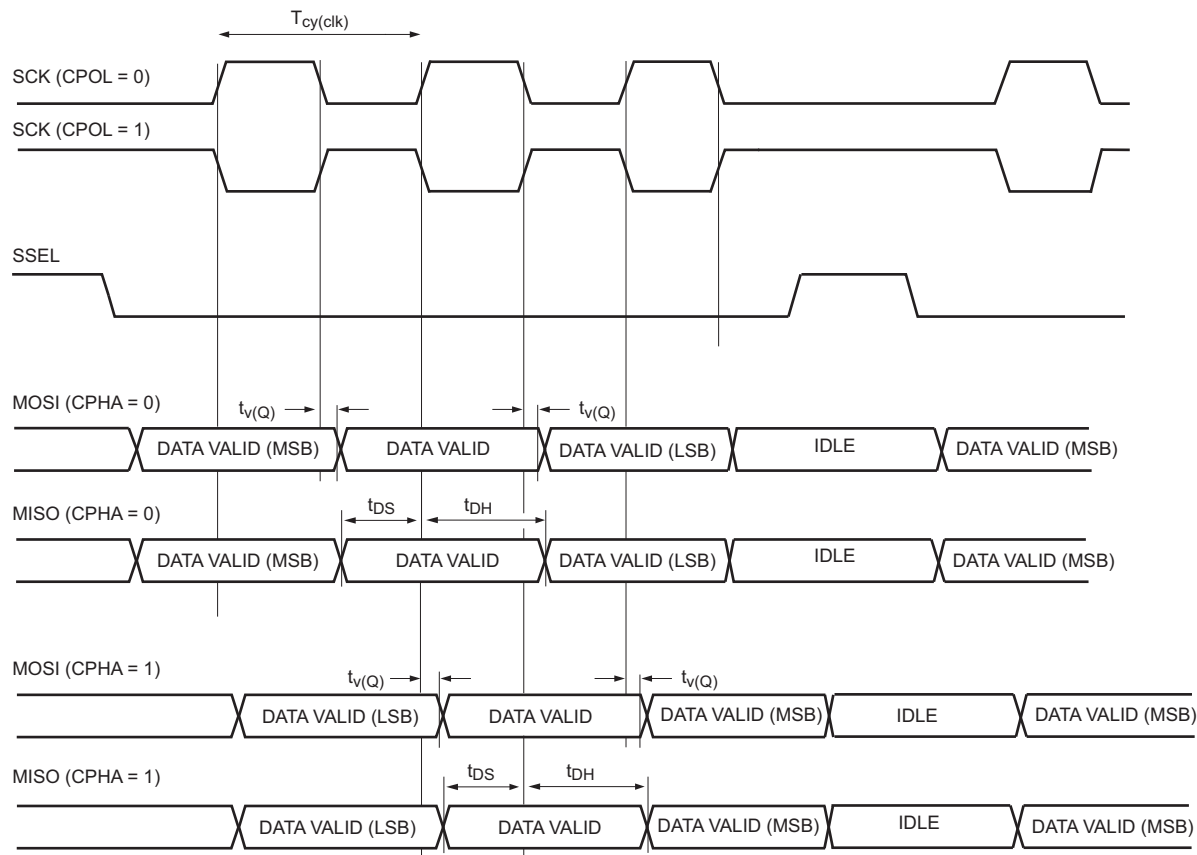
Fig 32. SPI master timing
