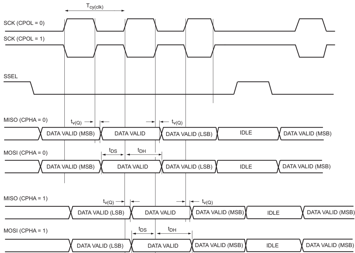
Fig 33. SPI slave timing
