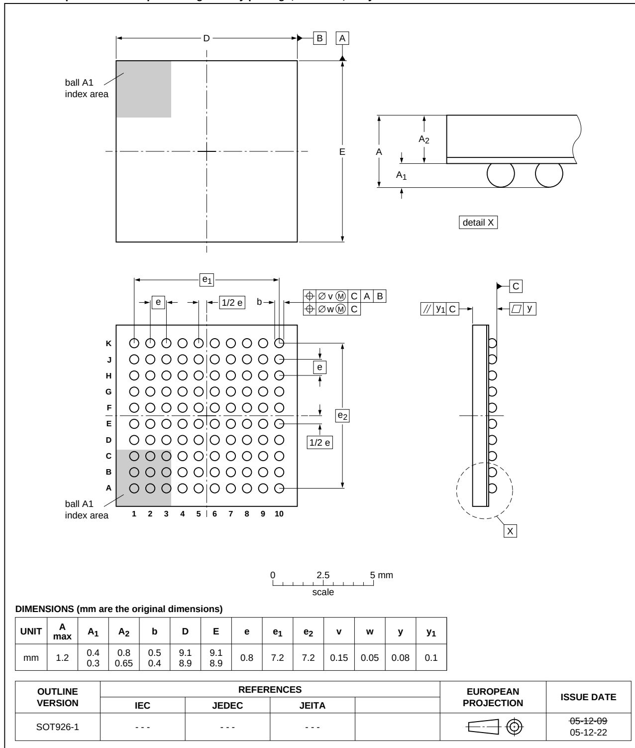
Fig 54. TFBGA100 package
