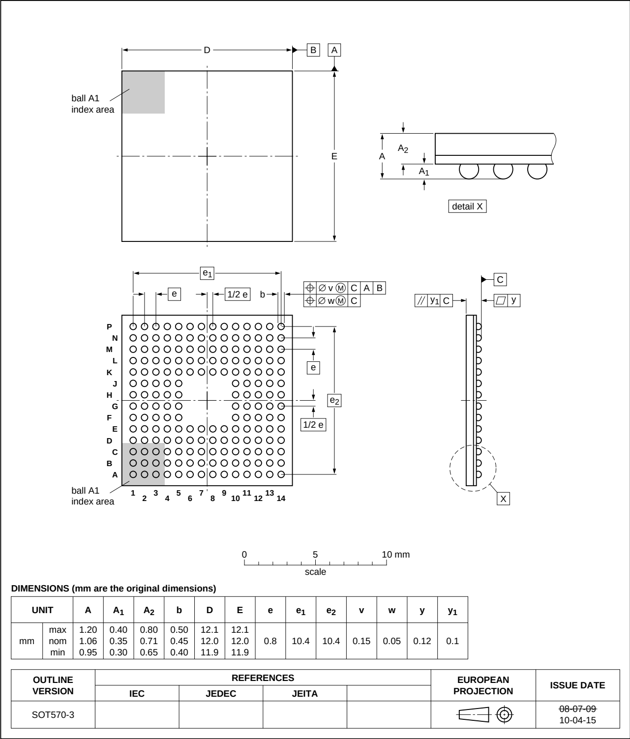
Fig 53. TFBGA180 package
