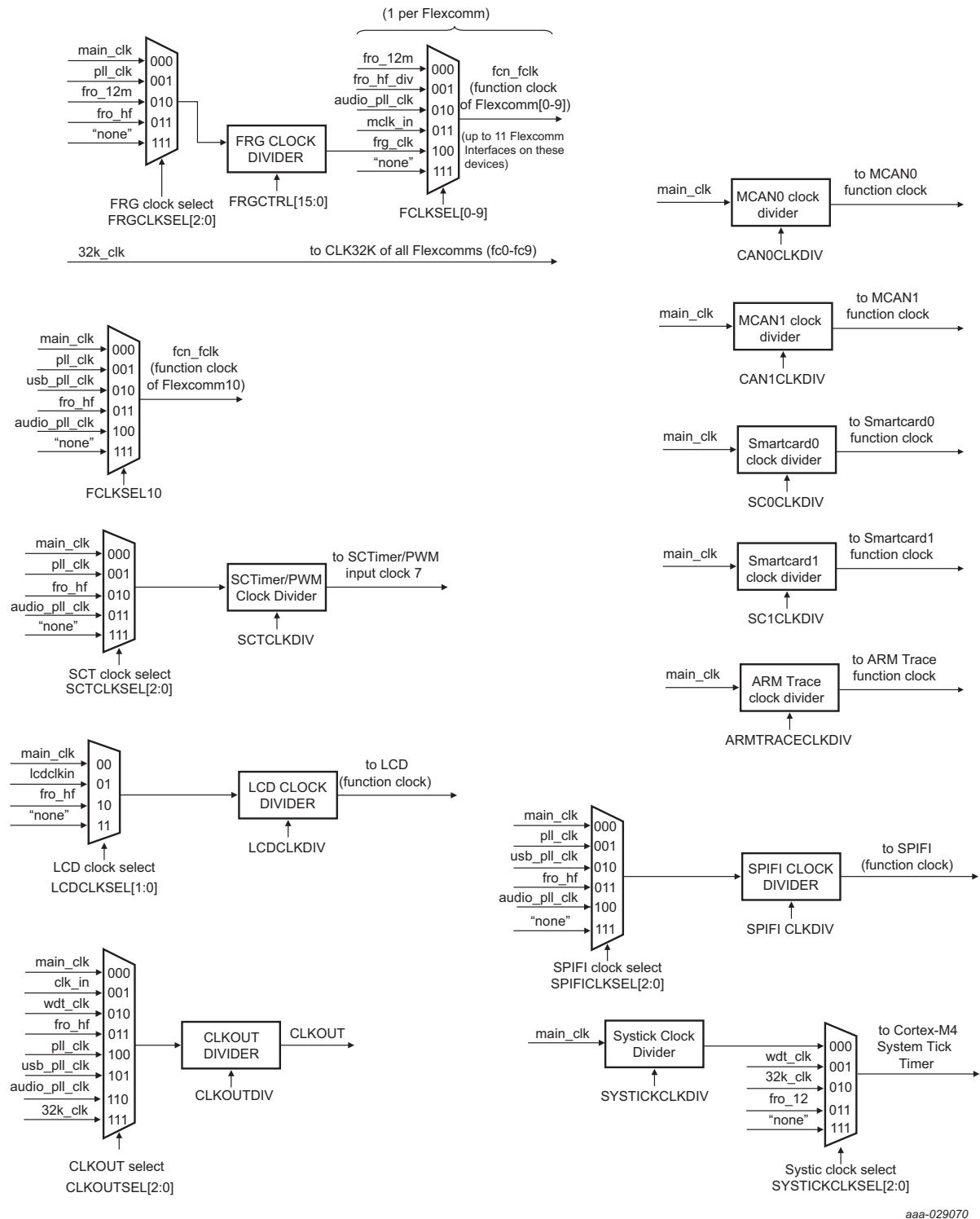
Fig 12. LPC540xx/LPC54S0xx clock generation (continued)
