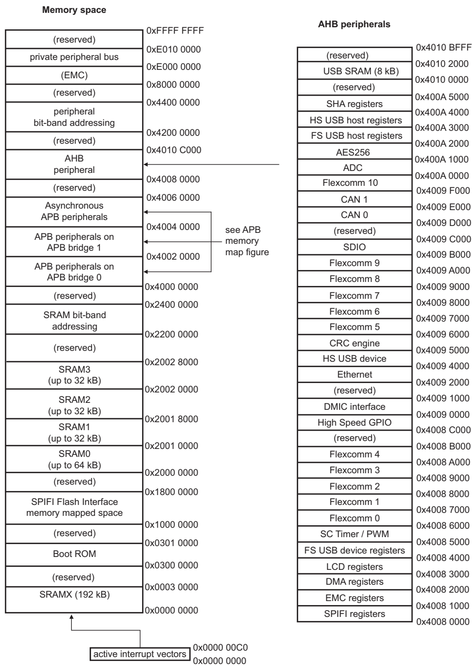
Fig 9. LPC540xx/LPC54S0xx Memory mapping
