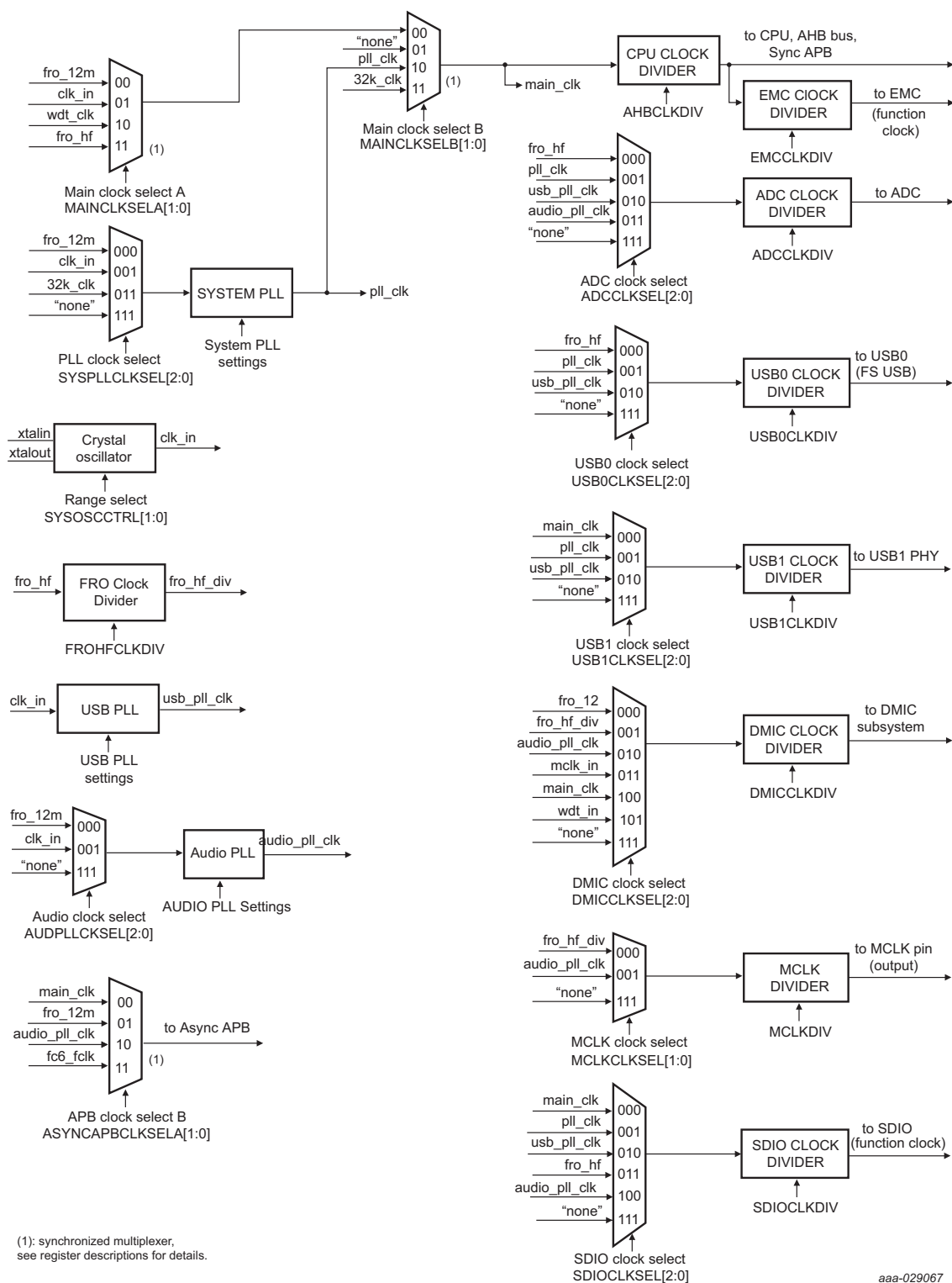
Fig 11. LPC540xx/LPC54S0xx clock generation
