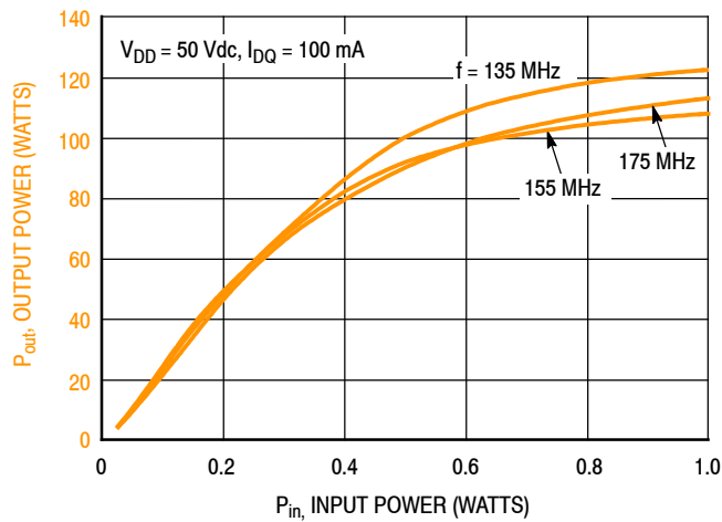
Figure 11. CW Output Power versus Input Power and Frequency
