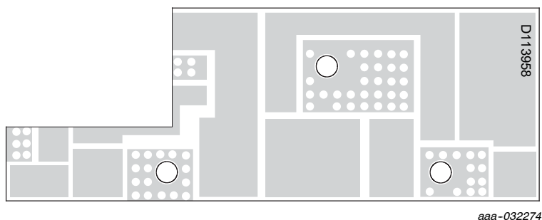
Figure 3. MRF101AN Compact Reference Circuit Board
