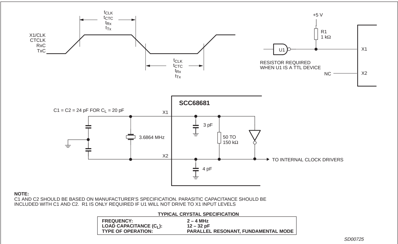
Figure 8. Clock timing
