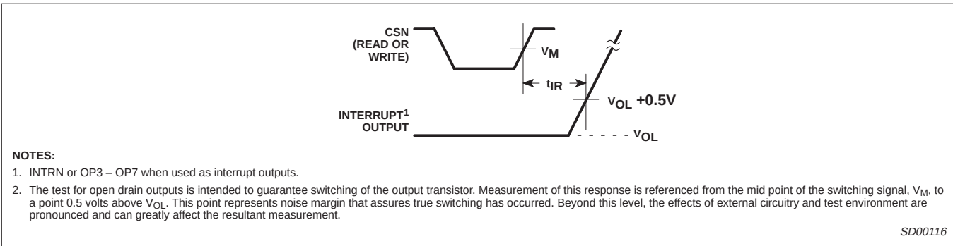
Figure 9. Interrupt timing
