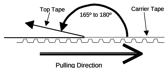
Fig.9 Peeling Strength
