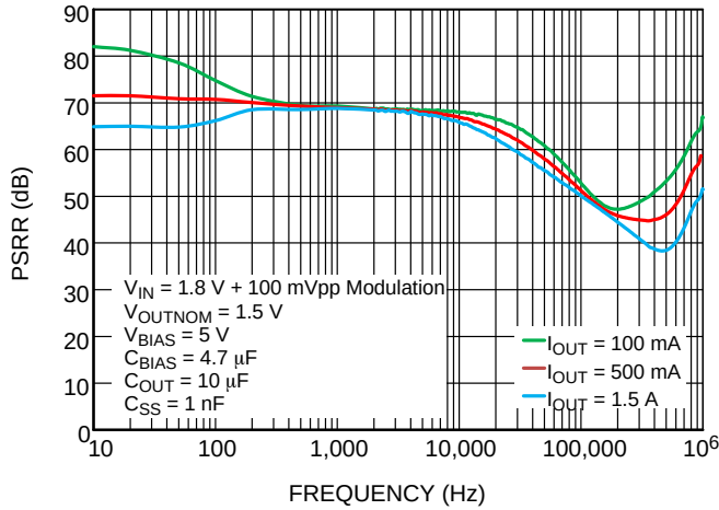
Figure 23. V_{IN} PSRR
