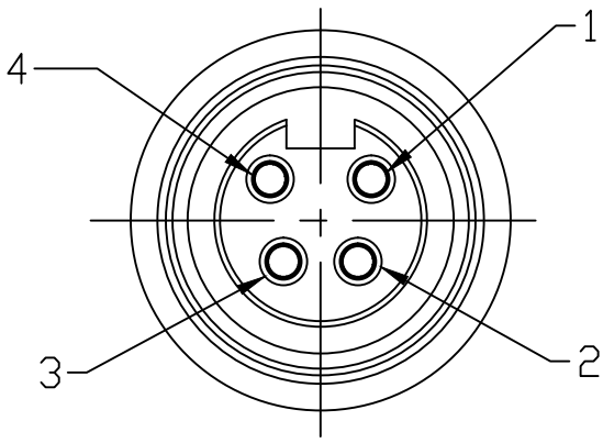
FEMALE INSERT FRONT VIEW
