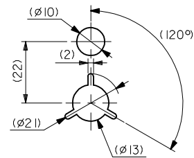
DETAIL G
