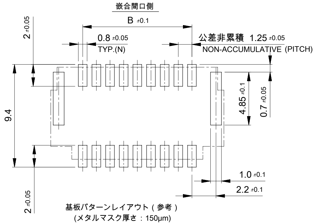
RECCOMENDED P.C.B. PATTERN LAYOUT (REF.) (METAL MASK THICKNESS : 150μm)
