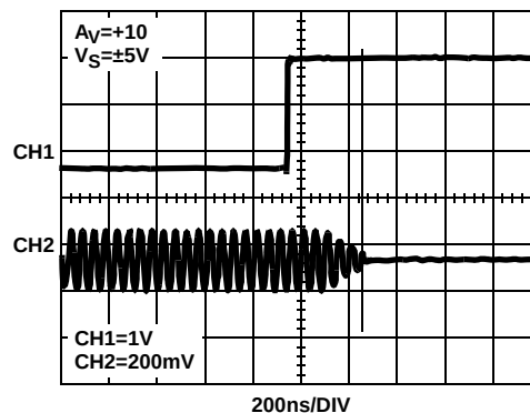
FIGURE 36. DISABLE RESPONSE/TURN-OFF TIME
