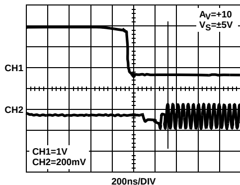
FIGURE 35. ENABLE RESPONSE/TURN-ON TIME
