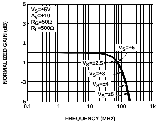
FIGURE 15. GAIN vs FREQUENCY FOR VARIOUS V_S \pm ( A_V = +10 )
