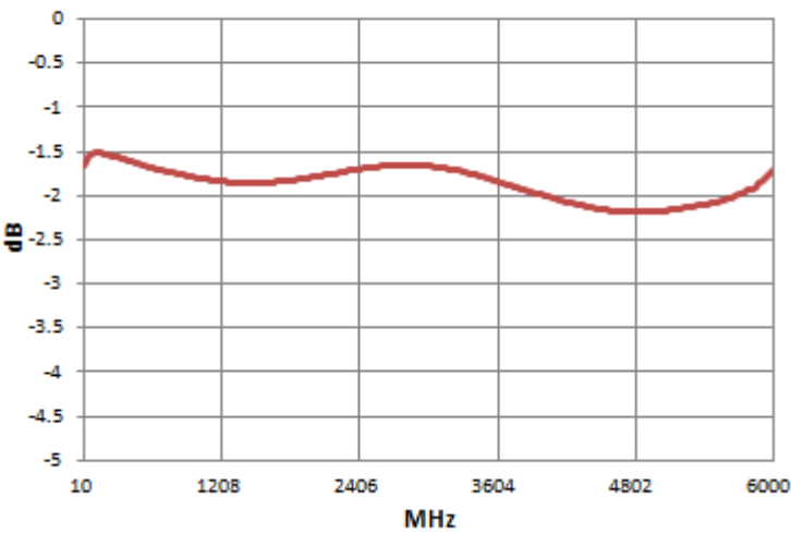
Insertion Loss
