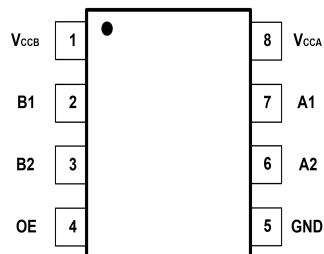
MS4553S (SOT-23-8L) Package
