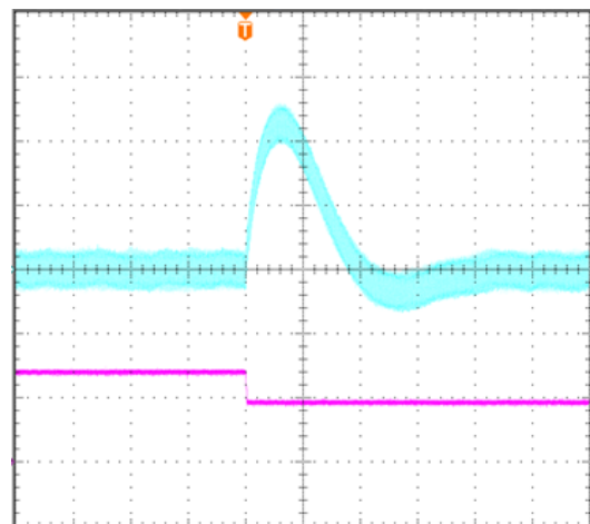
Figure 6: Transient Response
