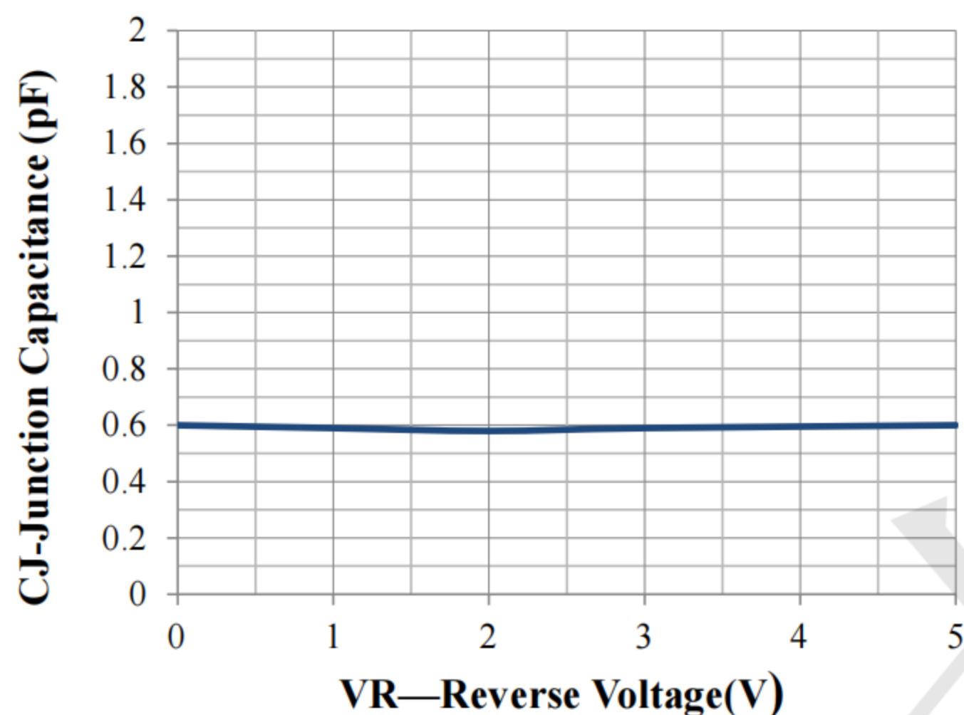
Junction Capacitance vs. Reverse Voltage
