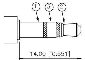
ø3.50 MATE PLUG
