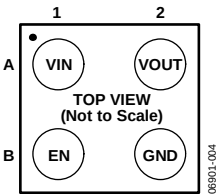
Figure 4. 4-Ball WLCSP Pin Configuration
