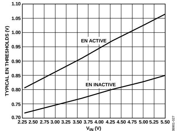
Figure 32. Typical EN Pin Thresholds vs. Input Voltage
