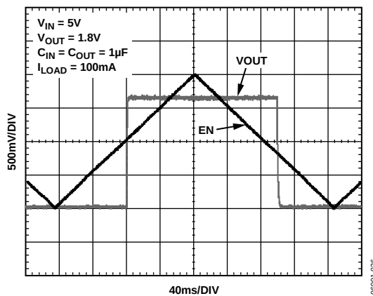
Figure 31. ADP121 Typical EN Pin Operation
