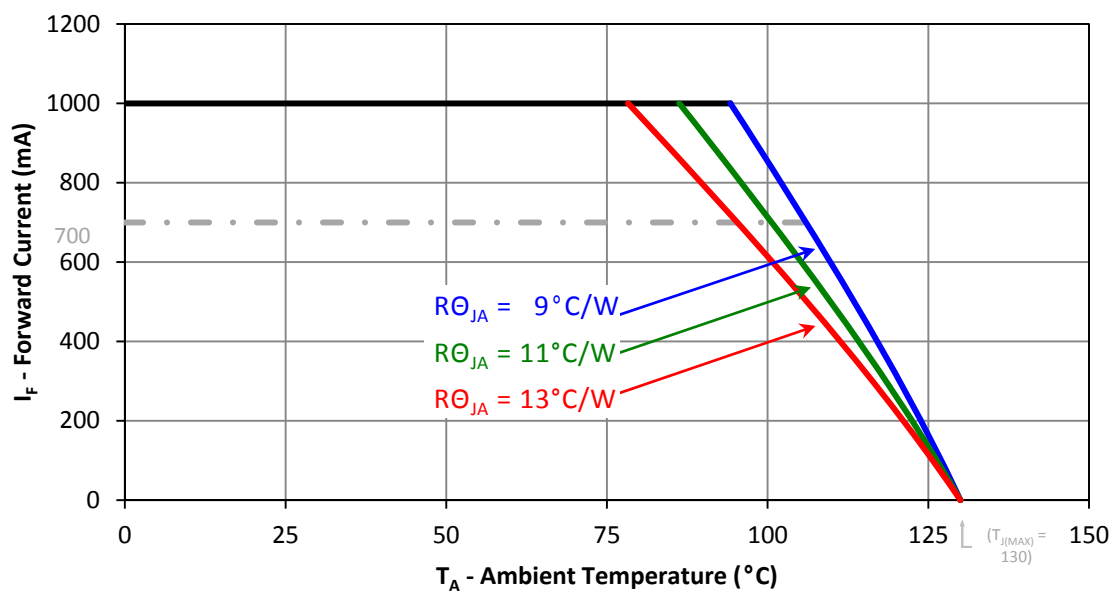
Figure 11: Maximum forward current vs. ambient temperature based on T_{J(MAX)} = 130^\circ\text{C} .
