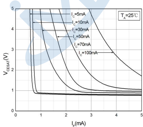
Fig.5 Collector-emitter Saturation Voltage vs. Forward Current
