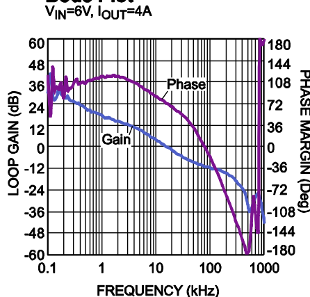
Bode Plot
