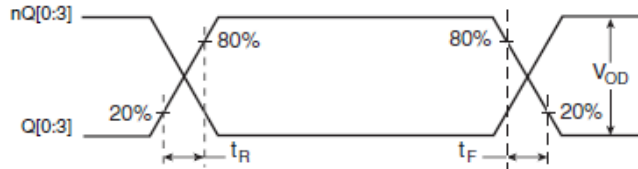
Figure 11. LVDS Output
