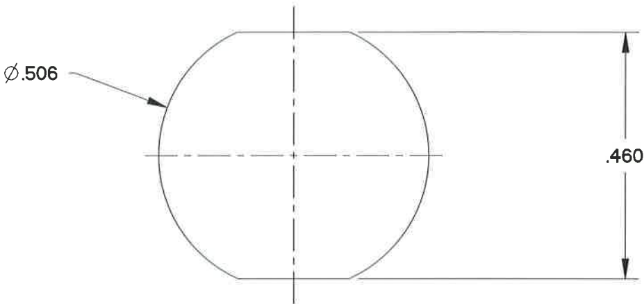
MOUNTING PANEL CUT OUT
