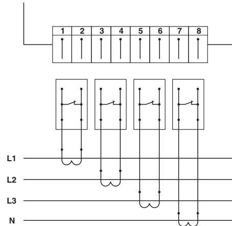
Circuit diagram
